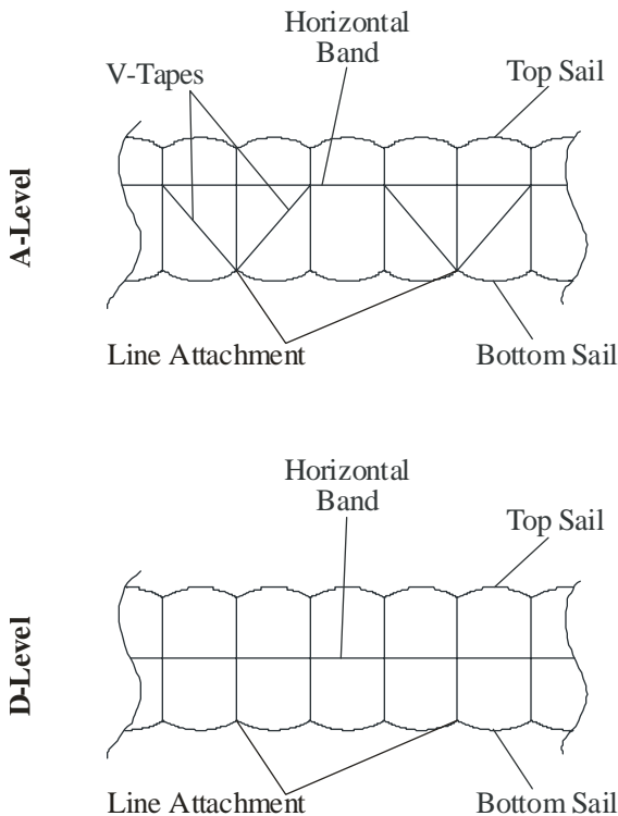
Illustration 1: UP Trango Honeycomb-V-Tape System
