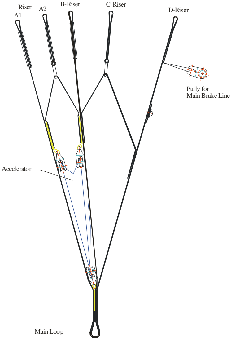
Illustration 2: UP Trango Riser
